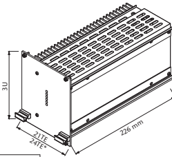
Standard Eurocassette (pluggable module for 19" sub-rack) approx. 2.5 kg *) applicable to 5 V output models
