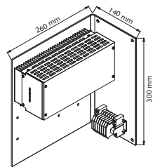
Optional Wall mount approx. 5.0 kg
