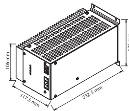
Optional Chassis mount approx. 3.0 kg
