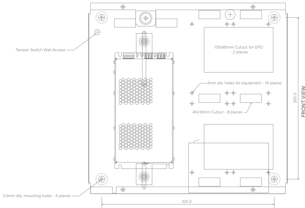
FRONT VIEW - COVER REMOVED
