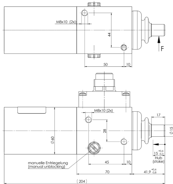
Dimension drawing
