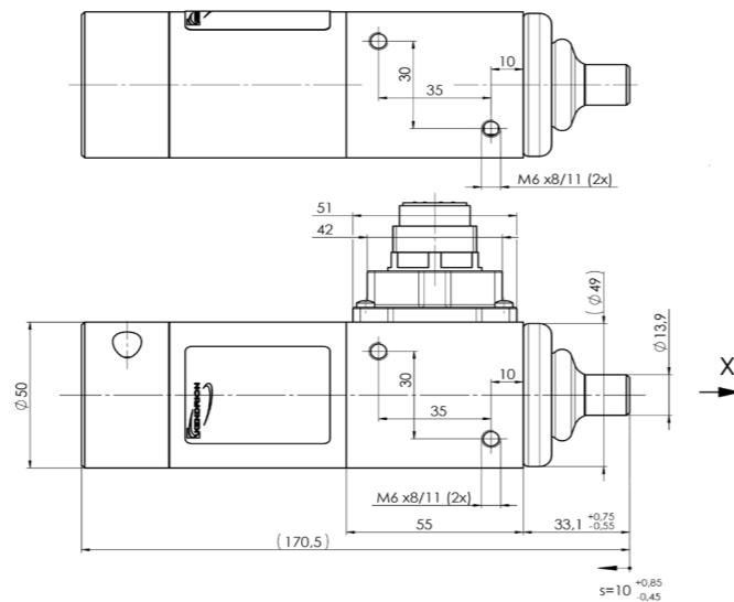
Dimension drawing
