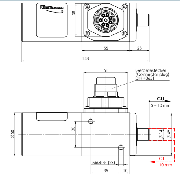
Dimension drawing
