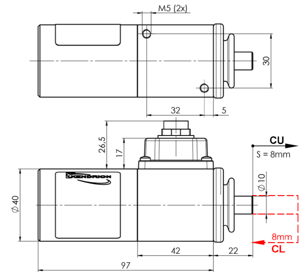
Dimension drawing
