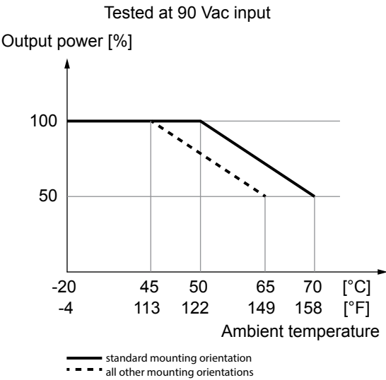
Fig. 8: Output power versus ambient temperature
