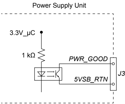
Fig. 17: Circuit diagram J3 Pin 9 (PWR_GOOD)
