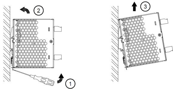
Fig. 2.2 Dismounting
