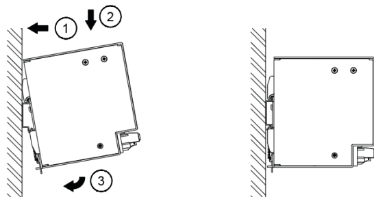
Fig. 2.1 Mounting
