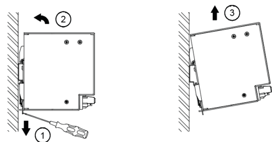
Fig. 2.2 Dismounting
