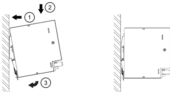
Fig. 2.1 Mounting
