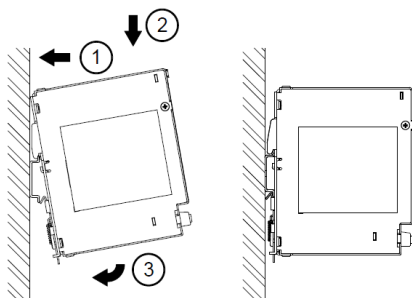
Fig. 6.1 Mounting
