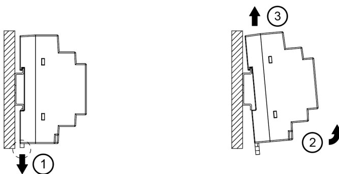
Fig. 2.2 Dismounting
