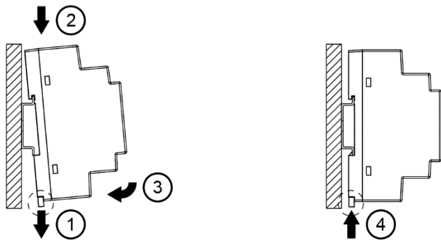
Fig. 2.1 Mounting
