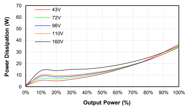
CHB300W-110S3V3-CMFC Pd Vs Po @25 Deg. C
