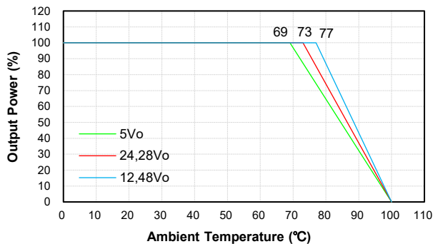
CHB200W-110SXX-CMFC(D) Derating Curve with Heat Sink (7.87x6.7x1.18inch) ( V_{in}=110V )
