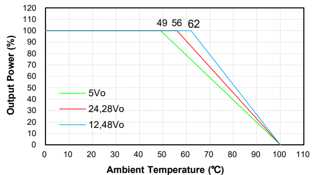
CHB200W-110SXX-CMFC(D)+HS(HD) Derating Curve ( V_{in}=110V )
