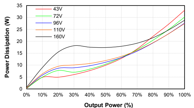
CHB200W-110S05-CMFC Pd Vs Po @25 Deg. C
