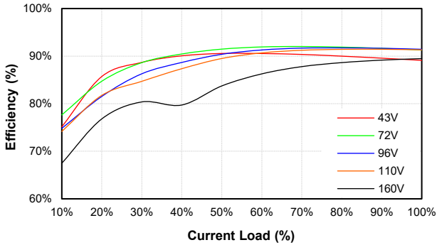
CHB200W-110S12-CMFC Eff Vs Io @25 Deg. C
