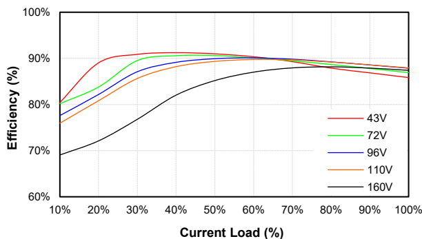
CHB200W-110S05-CMFC Eff Vs Io @25 Deg. C
