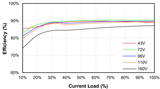
CHB200W-110S28-CMFC Eff Vs Io @25 Deg. C
