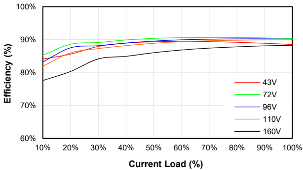
CHB200W-110S24-CMFC Eff Vs Io @25 Deg. C
