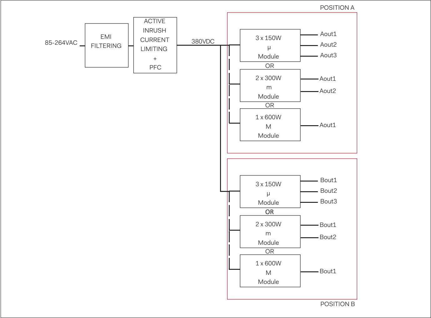
Block Diagram
